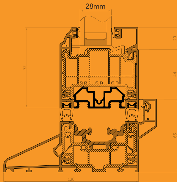
Decorative sash on 120mm integrated sill
