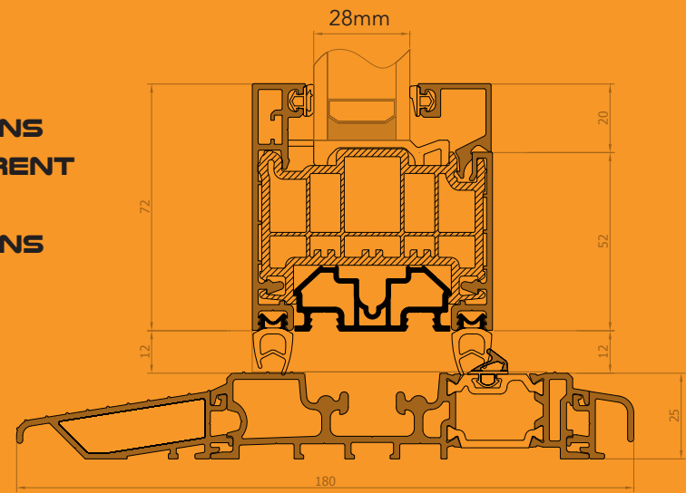
Square sash on Part M compliant low threshold
